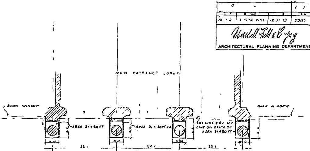
PLAN OF MAIN ENTRANCE OF STATE STREET
