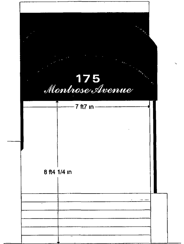
North Elevation
