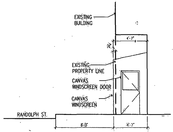
SIDE ELEVATION
