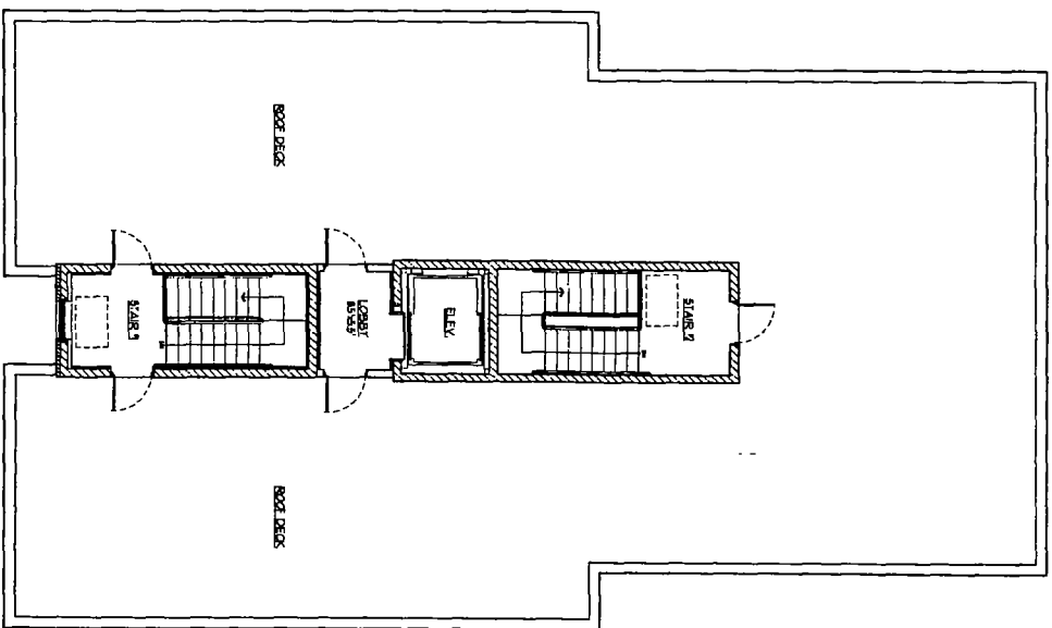
ROOF PLAN
