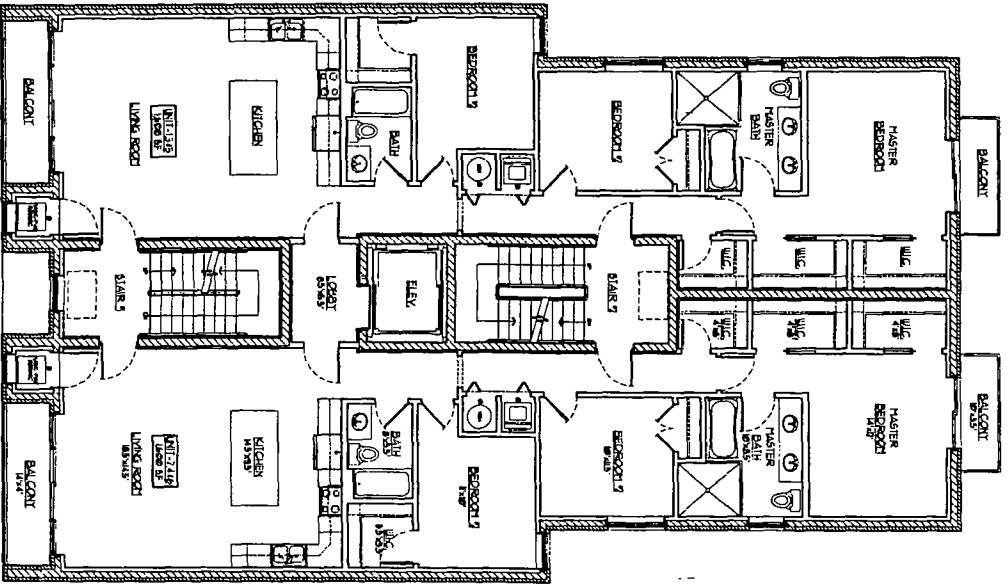
2-4TH FLOOR PLAN (TYP)
