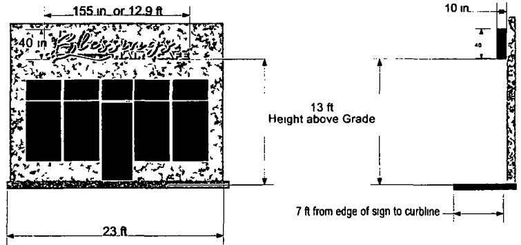
Standard Face Lit LED illuminated w/ Raceway SIDE VIEW
