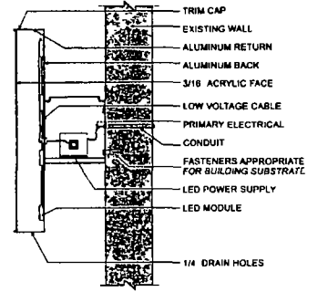
Standard Face Lit LED illuminated w/ Raceway SIDE VIEW
