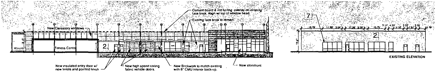
Building Elevations South
