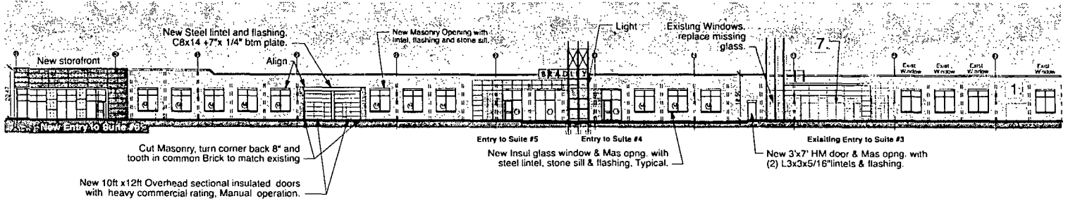
Building Elevation North
