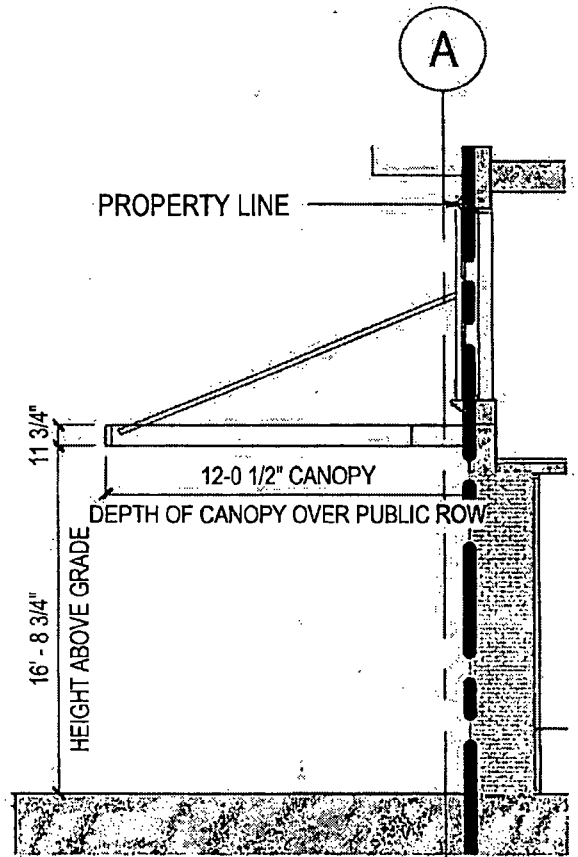
2 - ELEVATION VIEW
