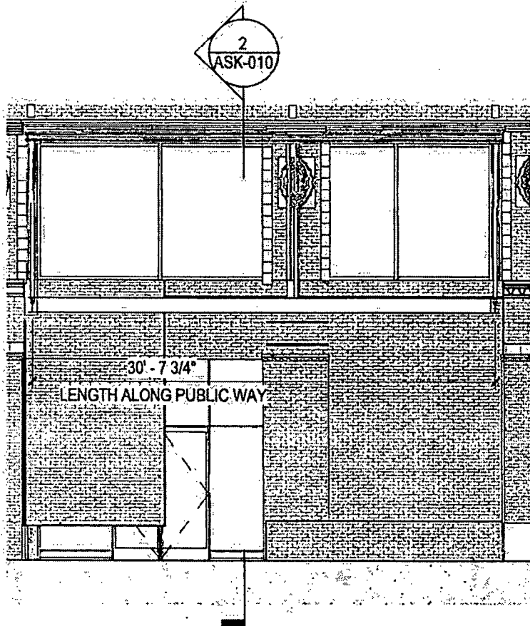
1 - ELEVATION VIEW
