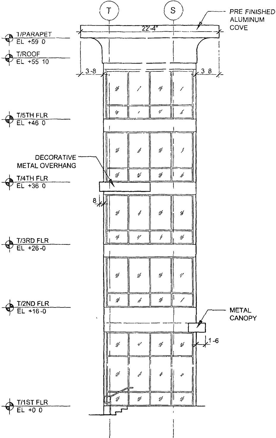
⑧ - NORTHEAST ELEVATION
