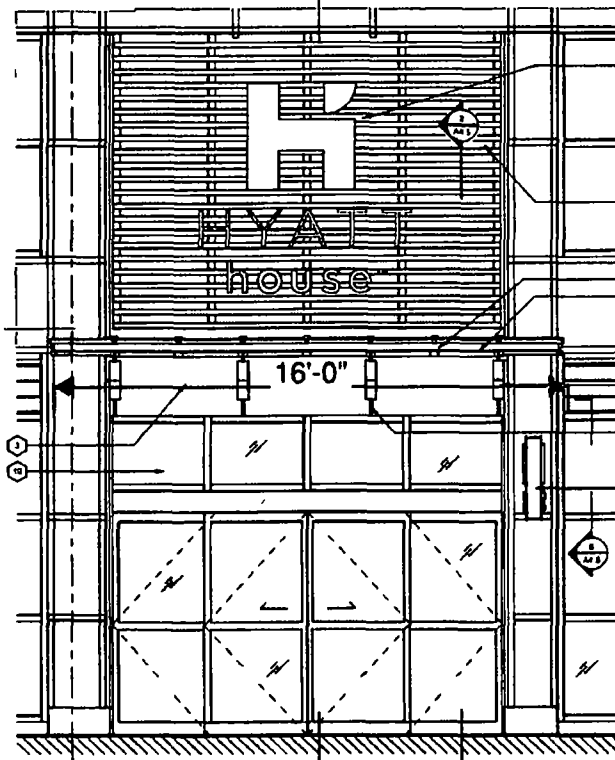
CANOPY ELEVATION
