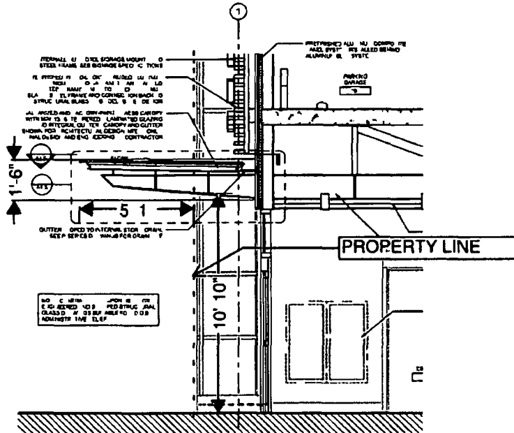
CANOPY SECTION
