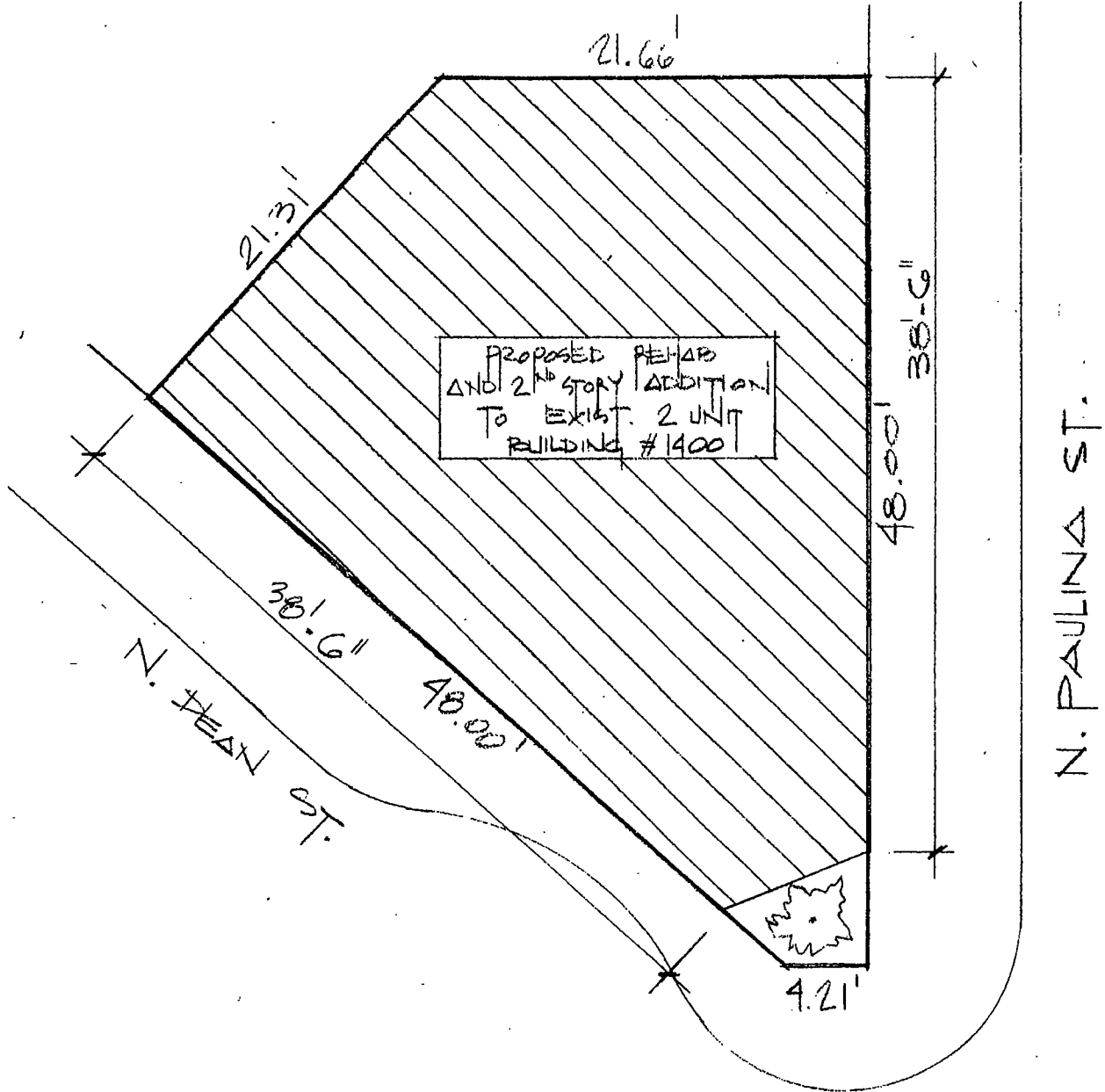
⊕ SITE PLAN 1/8" = 1'-0"
