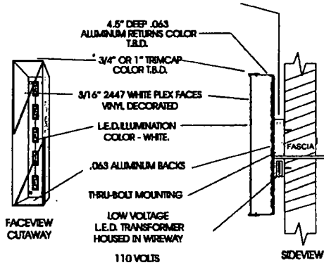
TYPICAL L.E.D. ILLUMINATED CHANNEL LETTER MOUNTED TO WIREWAY
