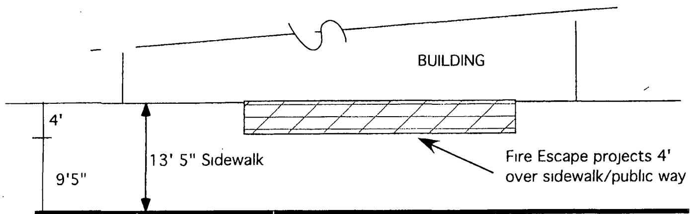
Partial Plan View N → Projecting Fire Escape Carpenter St
