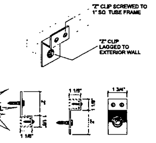
'Z' Clip Awning Attachments NTS
