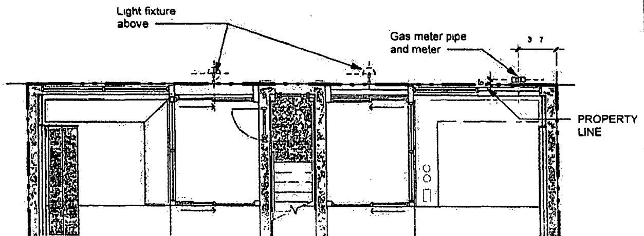
② PWU - Level 1 Gas meter location 1/8" = 1'-0"
