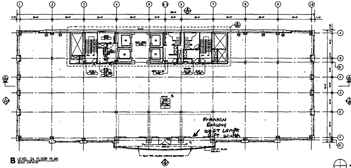
A LEVEL 25 FLOOR PLAN SCALE: 1/8" = 1'-0"
