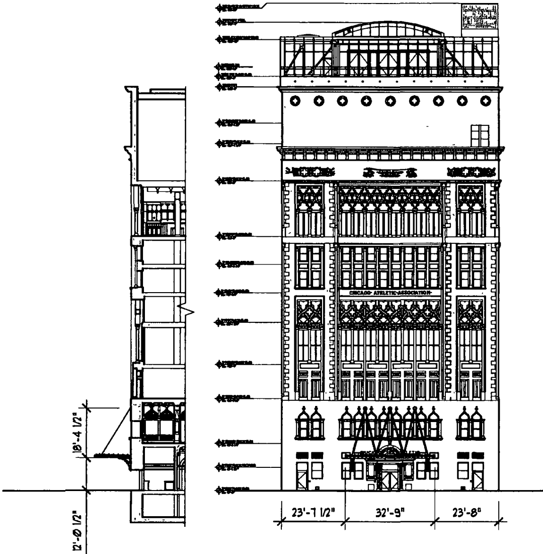
EAST ELEVATION / SECTION FIGURE 2
