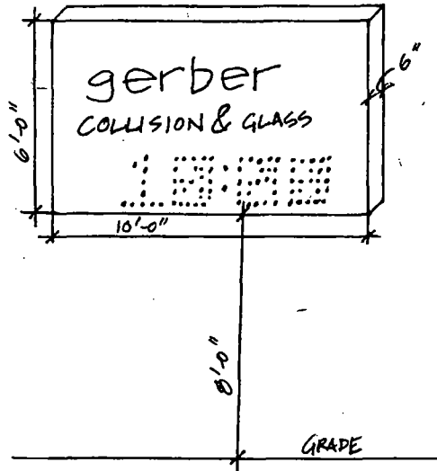
6'-0" x 10'-0" x 6" SIGN SCALE = 1/4" = 1'
