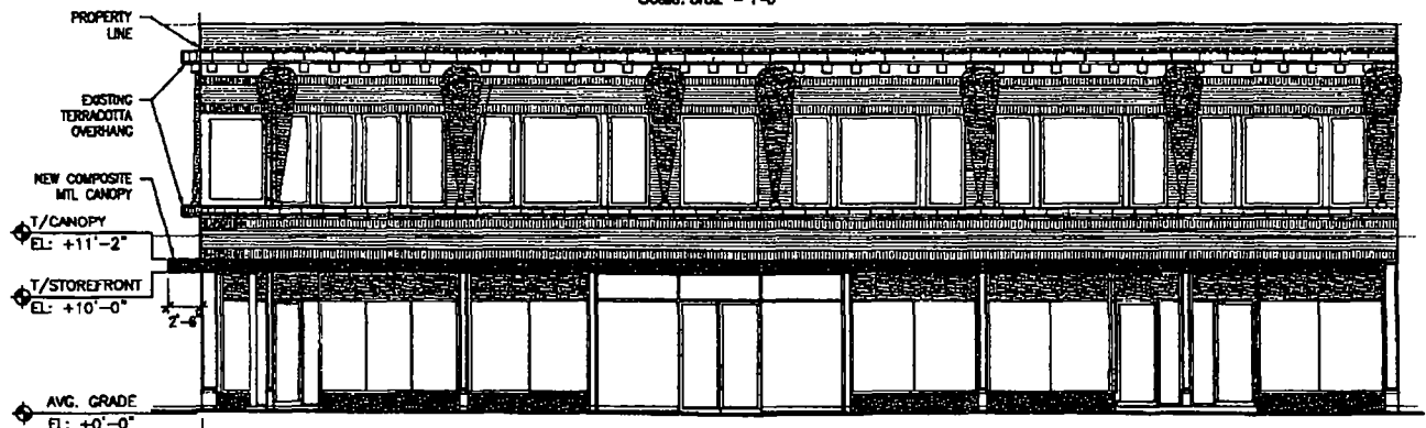
North Elevation
