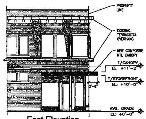
East Elevation
