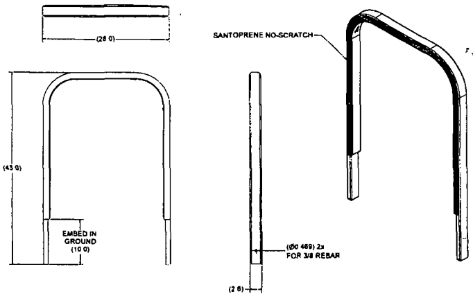
BIKE RACK DETAILS
