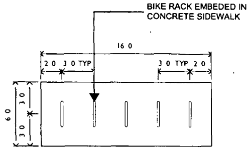
BIKE RACK PLAN DETAIL
