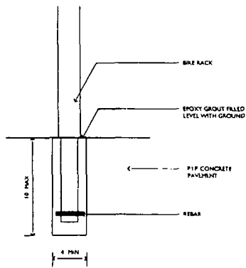
BIKE RACK EMBED DETAIL
