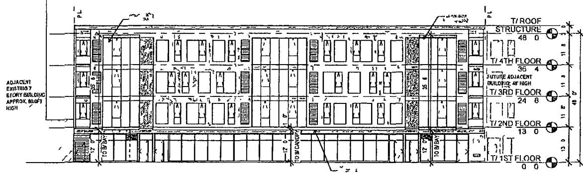
WEST ELEVATION SCALE 1/32 = 1 0
