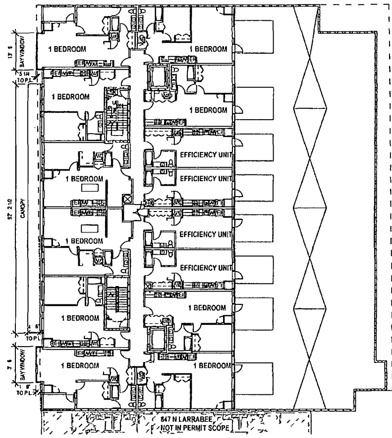
① 2ND FLOOR PLAN SCALE 1/32 = 1 0
