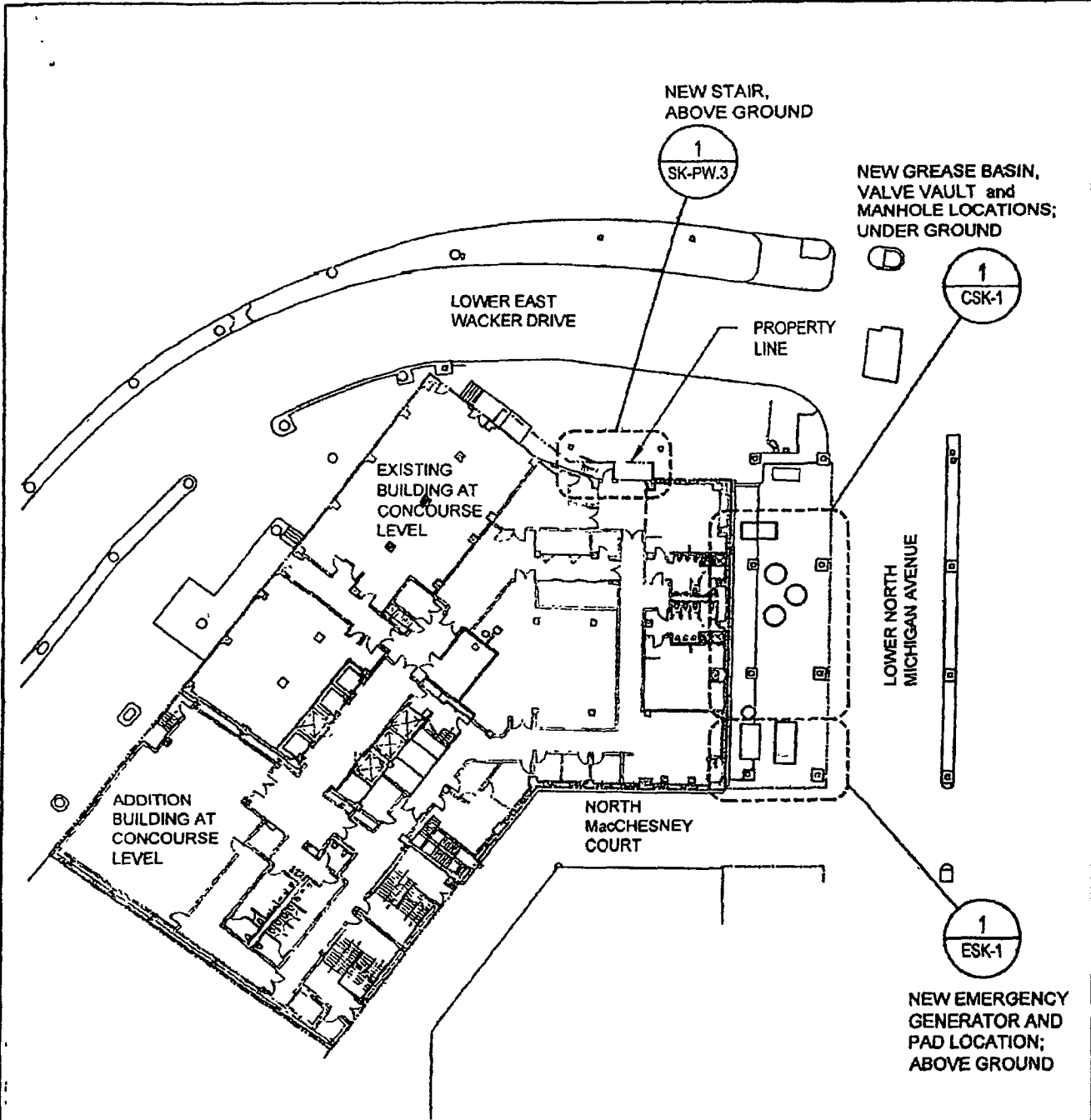
1 LOWER LEVEL SITE PLAN SCALE 1" = 40'-0" 0 20' 40' 80' 160'
