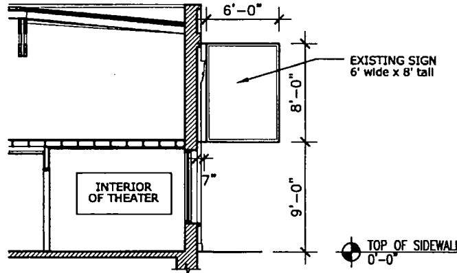
3 SECTION Looking West Down Belmont at Sign scale \frac{1}{8}'' = 1'-0''
