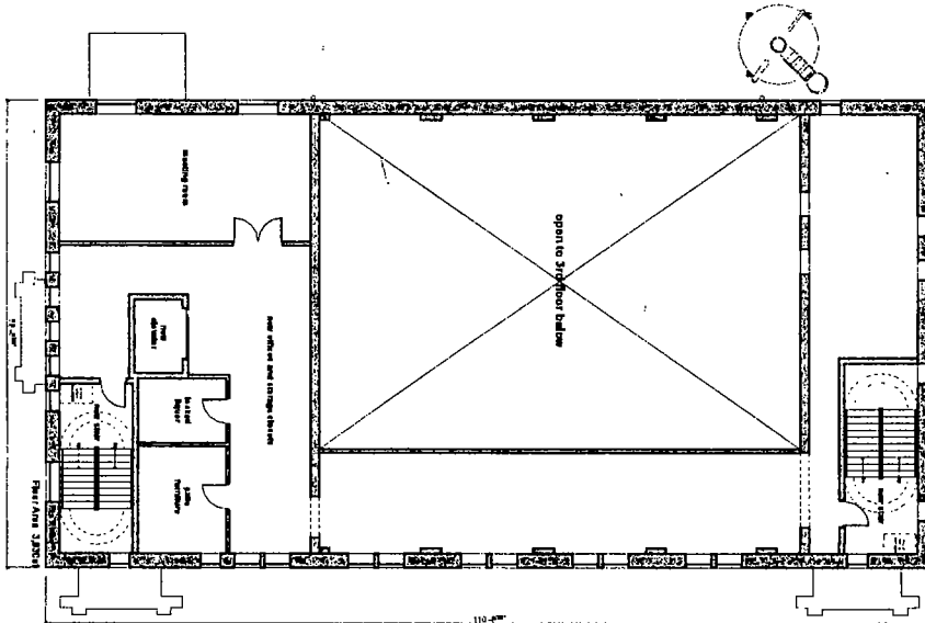
Proposed 4th Floor Plan SCALE 1/8" = 1'-0"
