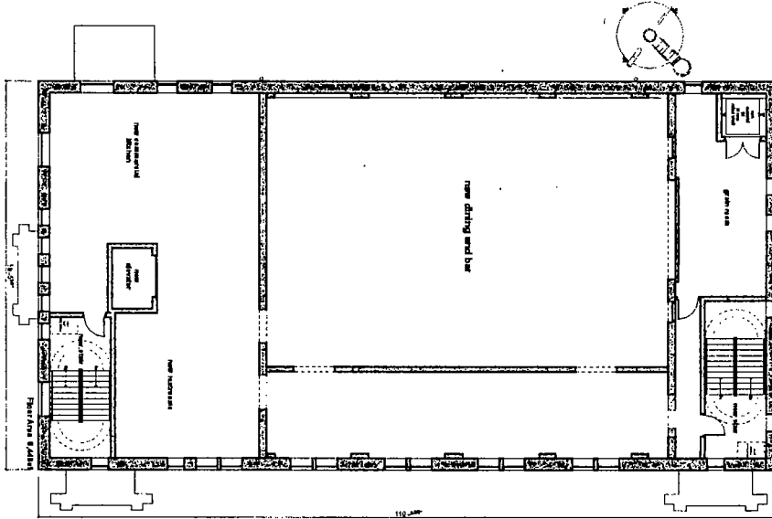
Proposed 3rd Floor Plan SCALE 1/8" = 1'-0"
