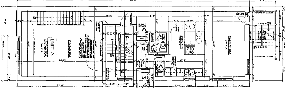
1ST FLOOR PLAN SCALE 1/8" = 1'-0"
