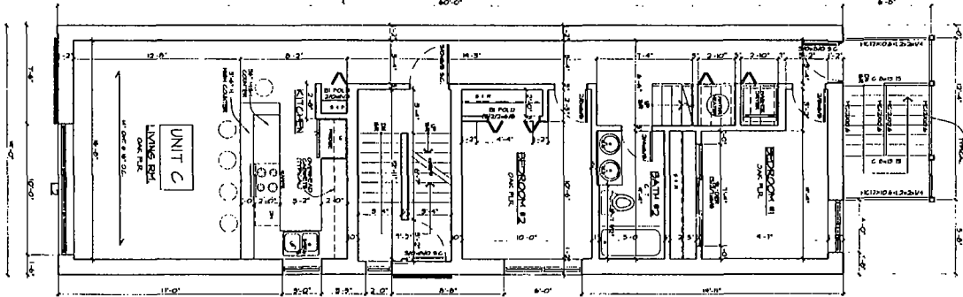
3RD FLOOR PLAN SCALE 1/8" = 1'-0"
