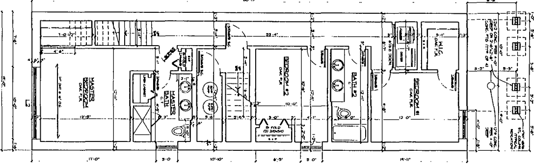
BASMENT PLAN SCALE 1/8" = 1'-0"
