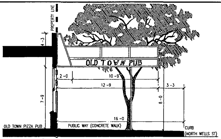
2 NORTH ELEVATION SCALE 3/16"=1'-0"
