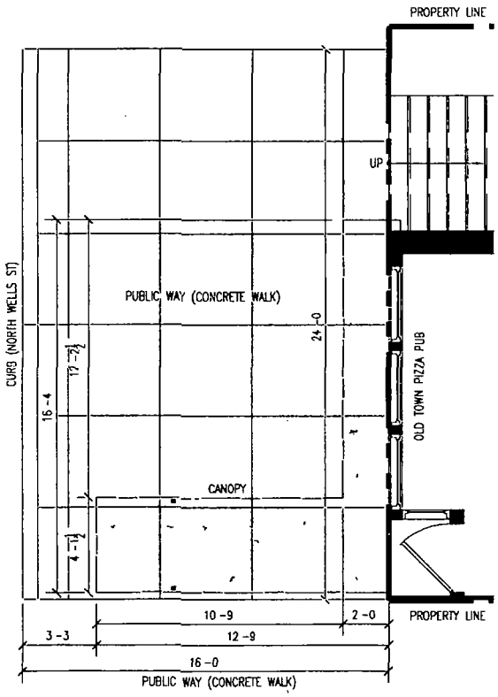
1 PLAN SCALE 3/16"=1'-0"
