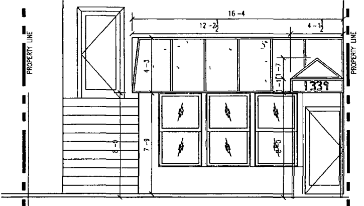
3 WEST ELEVATION SCALE 3/16"=1'-0"
