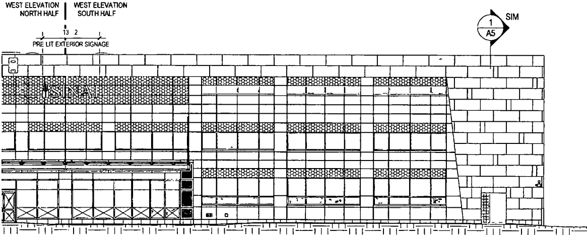
② WEST ELEVATION - SOUTH HALF 1/16 = 1-0
