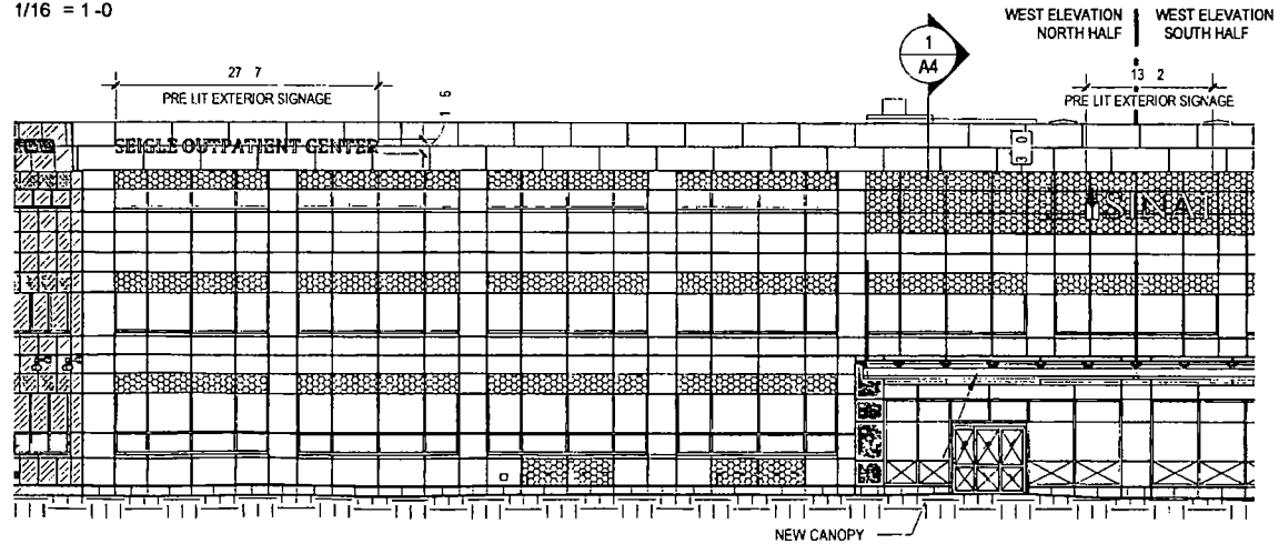
① WEST ELEVATION - NORTH HALF 1/16 = 1-0
