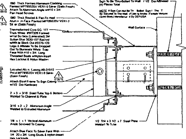
SECTION THROUGH CASE AT CLADDING PLAN VIEW SCALE 3 = 1
