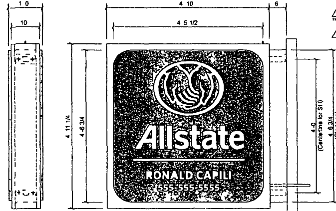
ELEVATION ALLST.FLG.25 25 SQ.FT.FLAG SIGN SCALE 3/4 = 1
