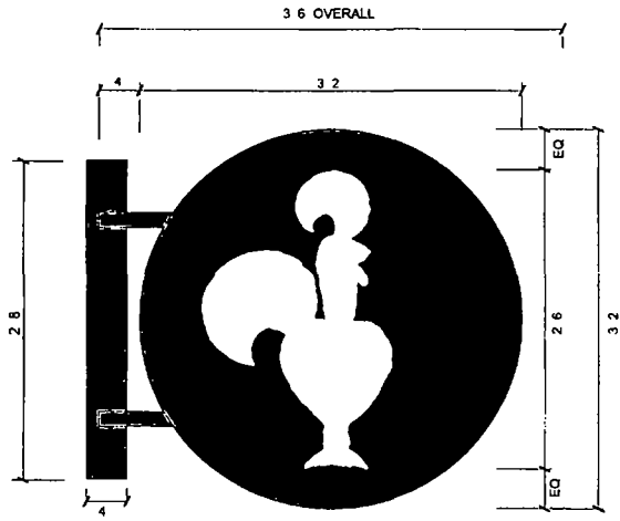
FACE VIEW
