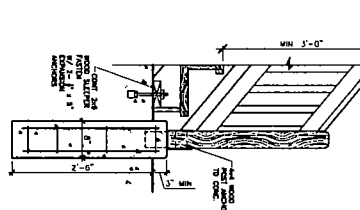
12 (F-2) CONCRETE PIER DETAIL SCALE 1/4" = 1'-0"
