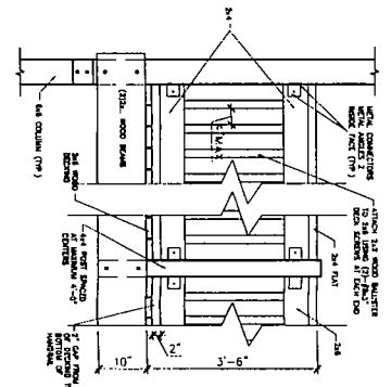
11 RAILING ELEVATION SCALE 1/4" = 1'-0"
