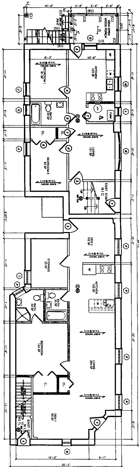
ARCH. FIRST FLOOR PLAN 3/16" = 1'-0"
