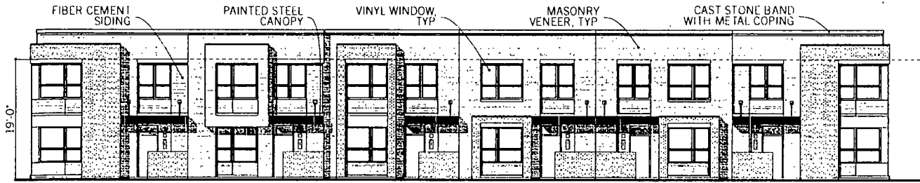
Front Elevation 1
