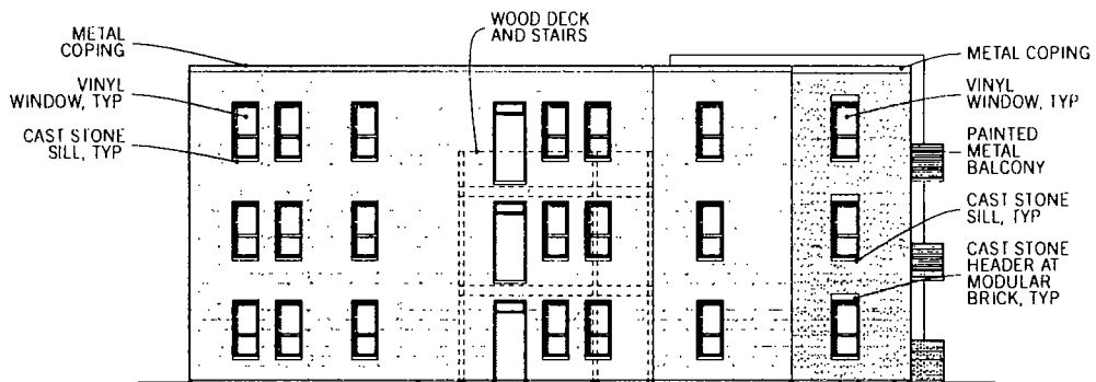
South Elevation
