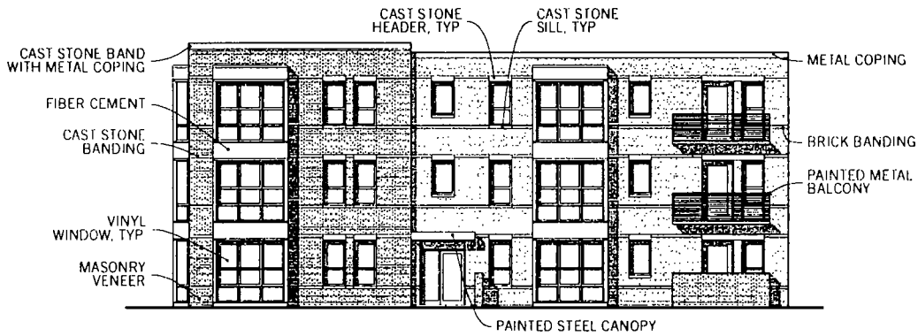
West Elevation
