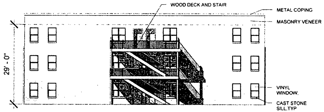
2 Elevation 2 (Back) 1" = 20'-0"
