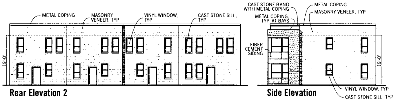
Front Elevation 2
