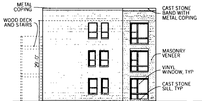
G1 - Side Elevation
