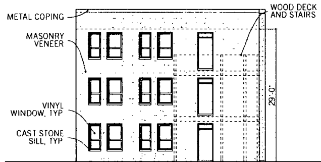
G1 - Rear Elevation
