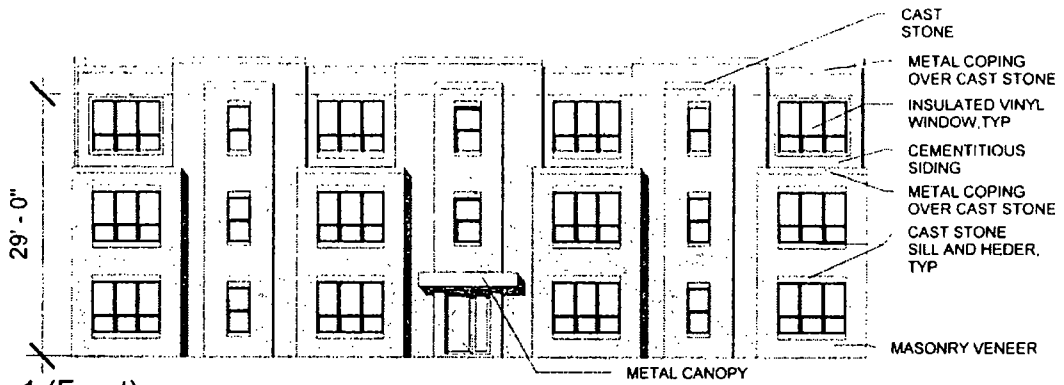
1 Elevation 1 (Front) 1" = 20'-0"
