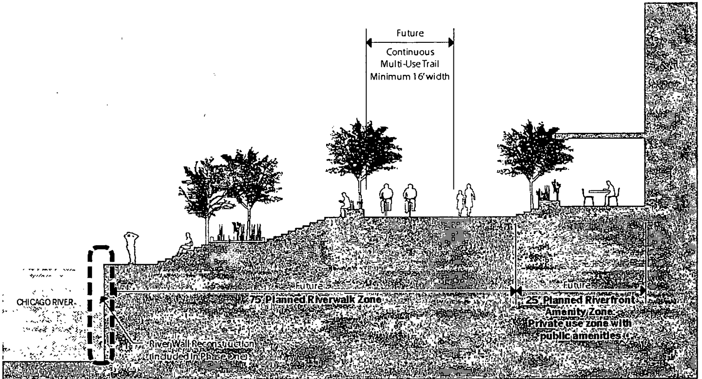
River Wall Section
