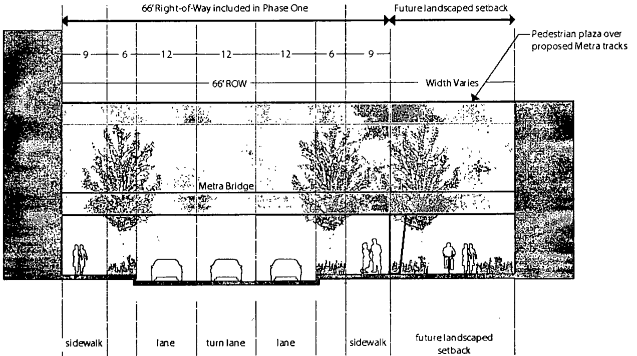
15th Street Section
