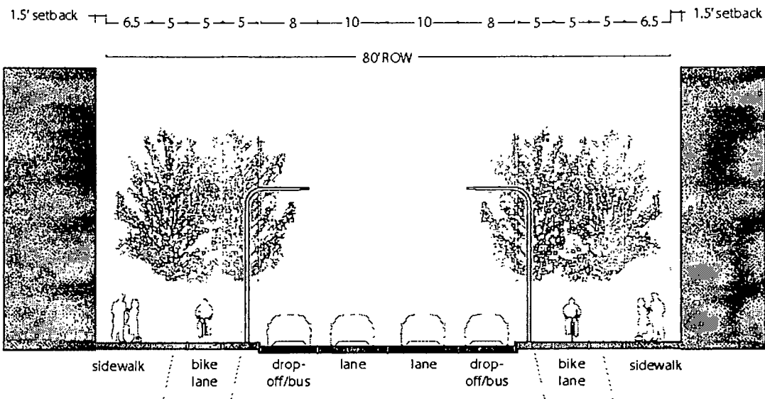
Wells Street Section
