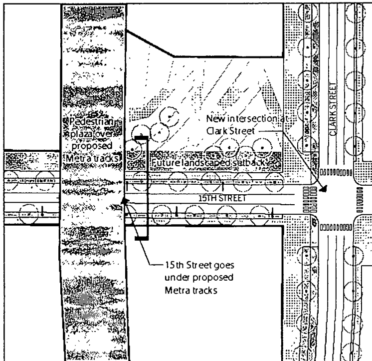
15th Street Typical Plan
