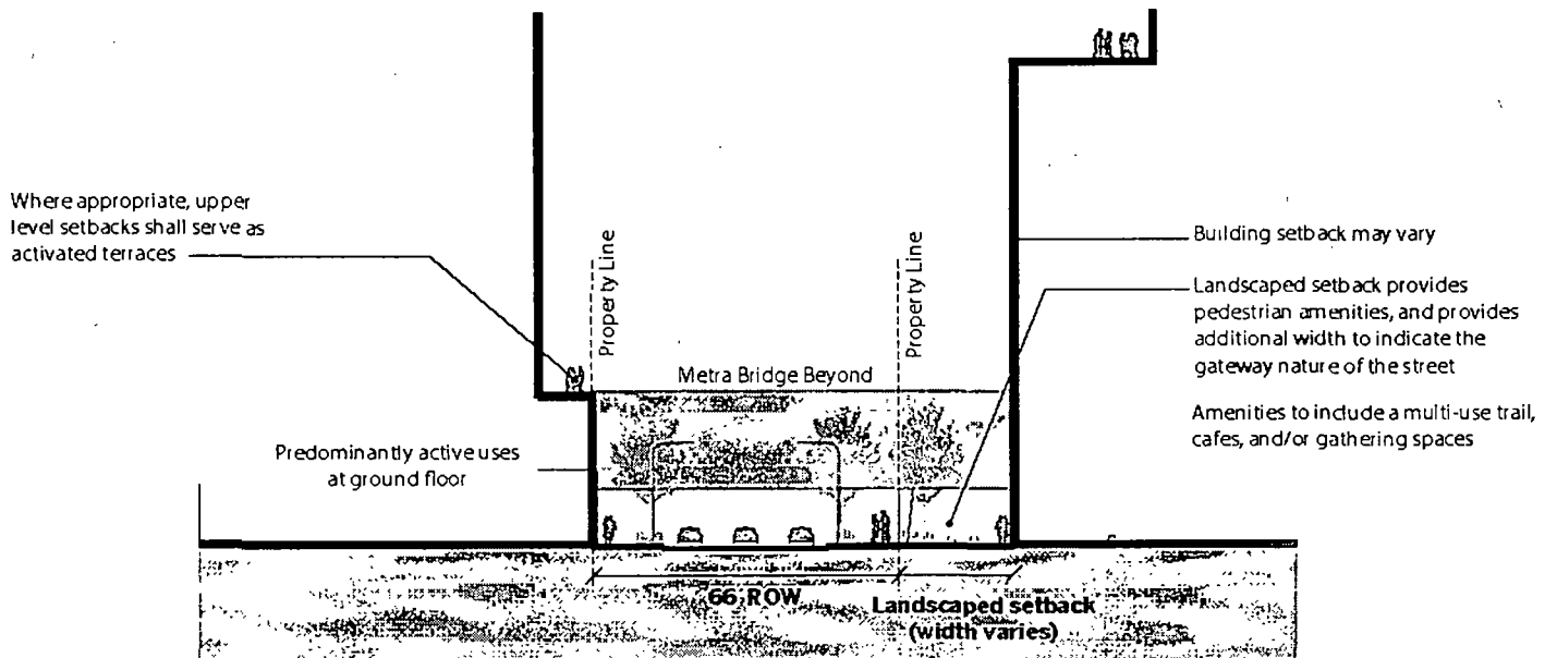
15th Street Section (facing west)
