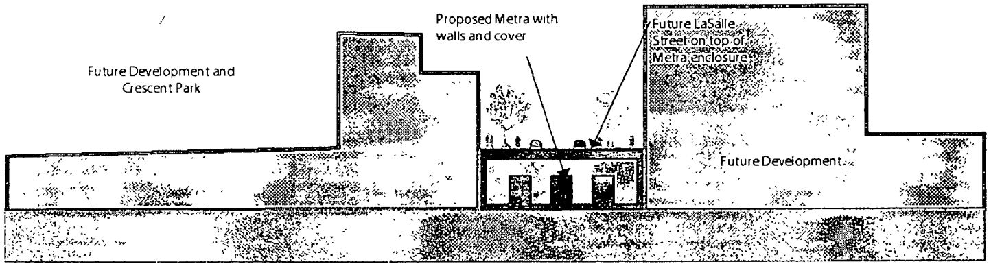
A. Metra Section, Typical
