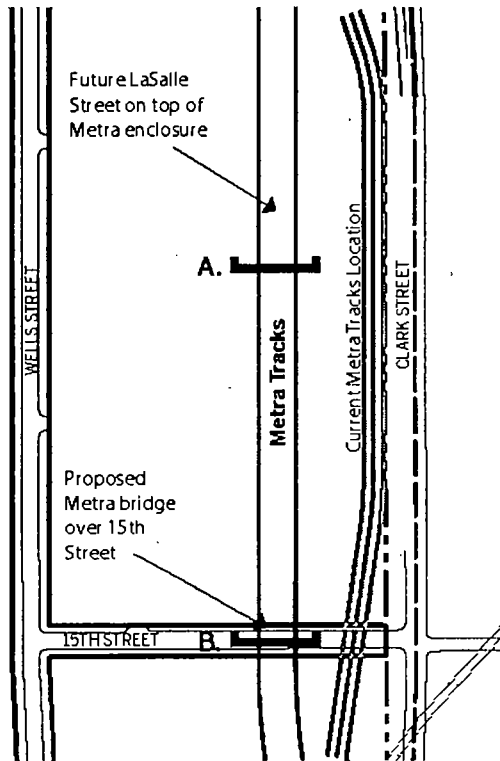
Metra Typical Plan
