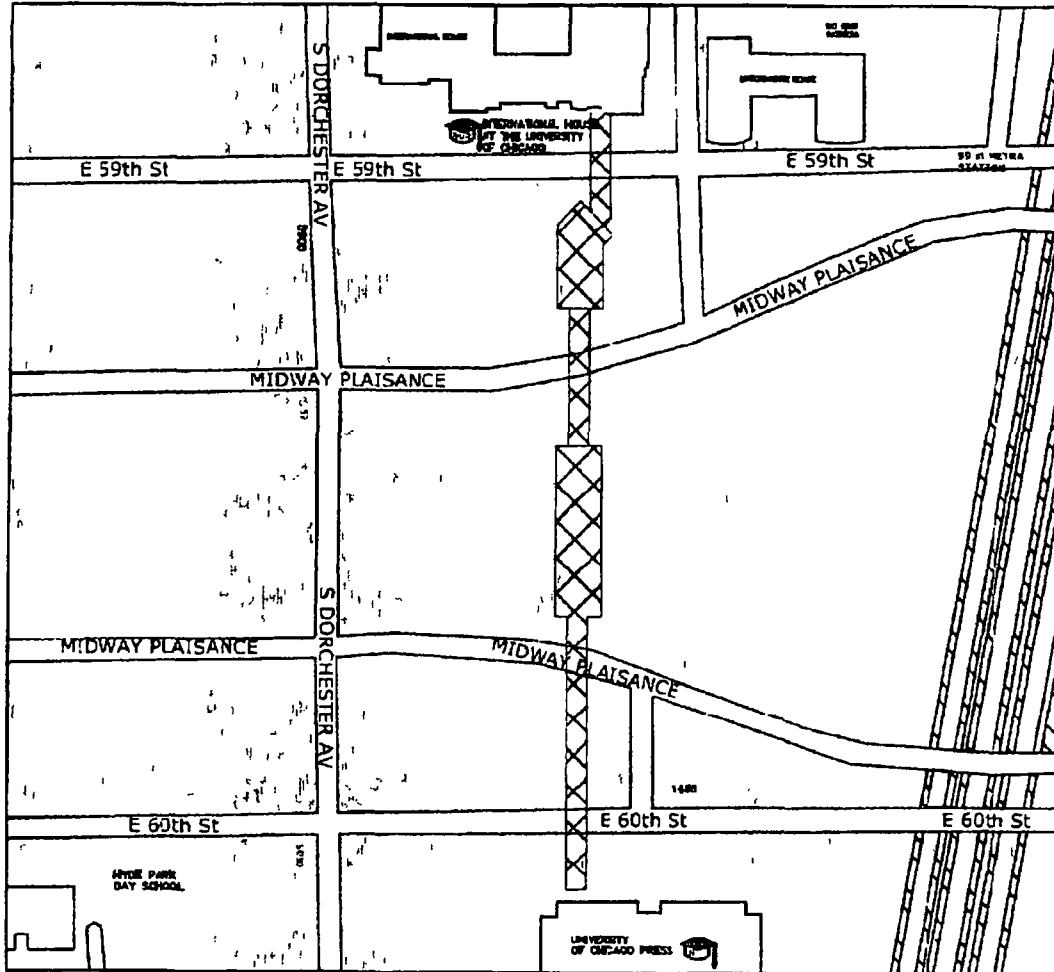
Chilled Water Lines at 59 th - 60 th /Dorchester University of Chicago
