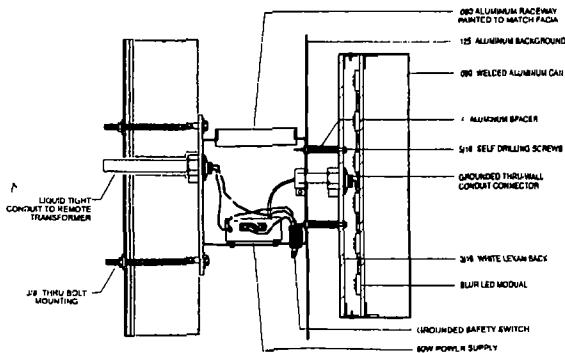
Typical U.L. Reverse Channel Letters with LEDs Mounted on Raceway Not to scale
