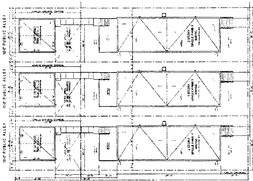
S. CHARLIE AVE SITE/ROOF PLAN
