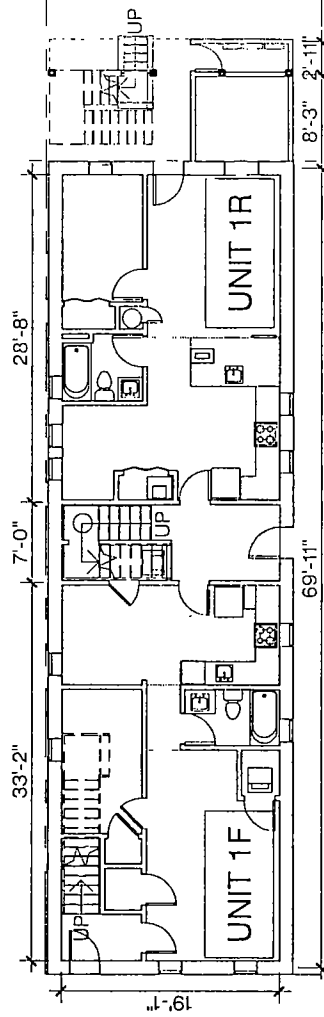
1st Level Plan (Existing)
