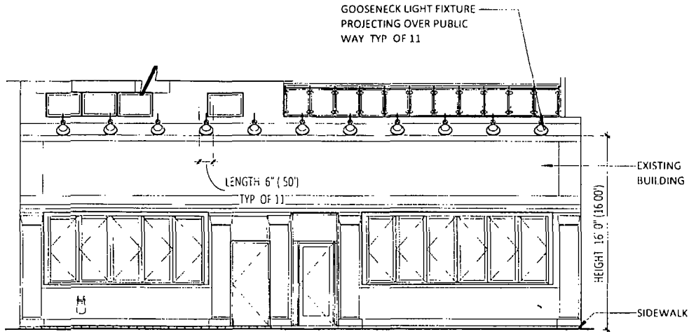
1 FRONT ELEVATION -PUBLIC WAY PERMIT 1/8" = 1'-0"
