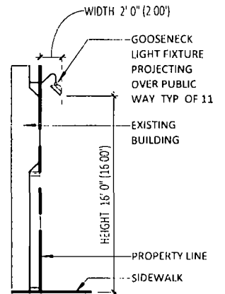
2 SIDE ELEVATION 1/8" = 1'-0"
