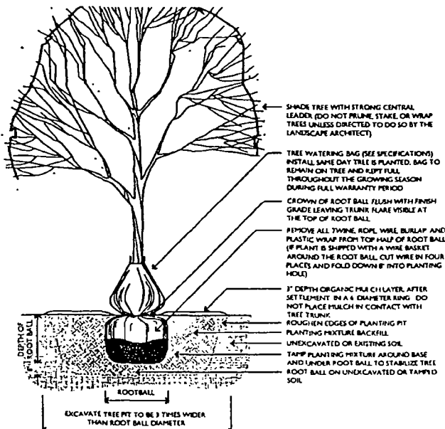
2 TREE INSTALLATION DETAIL 3/8" = 1'-0"
