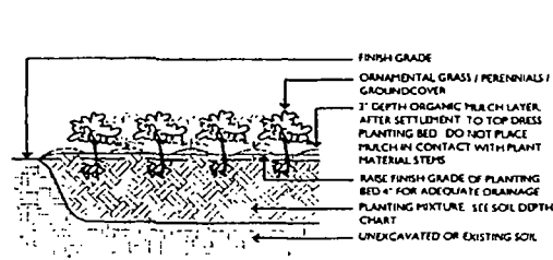
3 GROUND COVER/PERENNIAL INSTALLATION DETAIL 3/8" = 1'-0"
