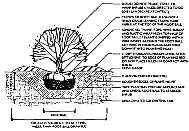
4 SHRUB INSTALLATION DETAIL 3/8" = 1'-0"
