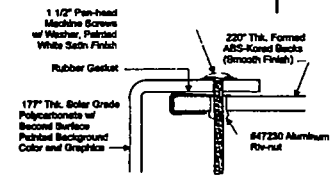
Face Mounting Detail Scale NTS
