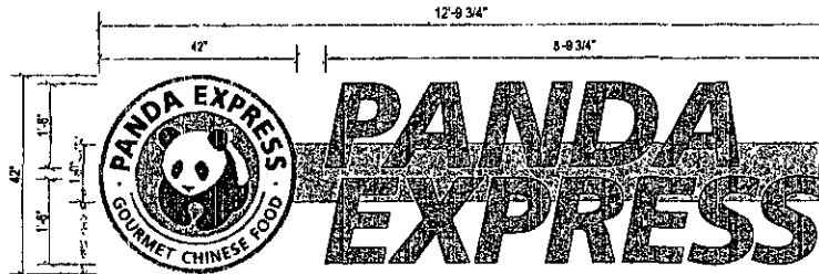
Sign Layout Detail Scale 1/2" = 1'-0"
