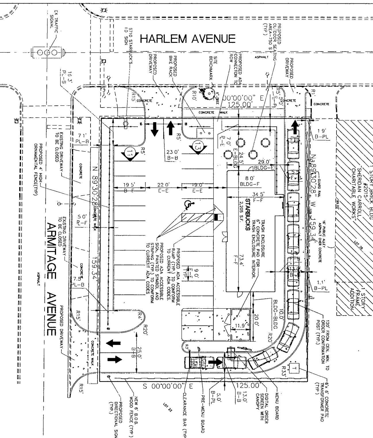
SITE PLAN #16
