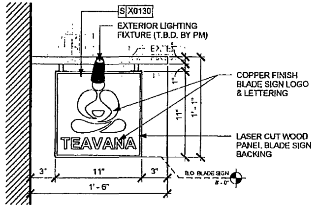
3 BLADE SIGN DETAIL (ELEVATION) Scale: 1 1/2" = 1'-0"
