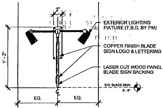
2 BLADE SIGN DETAIL (SIDE VIEW) Scale: 1 1/2" = 1'-0"
