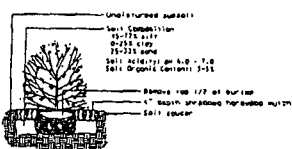
Detail: Shrub Planting
