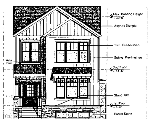
30 ft Lot - Option 5
