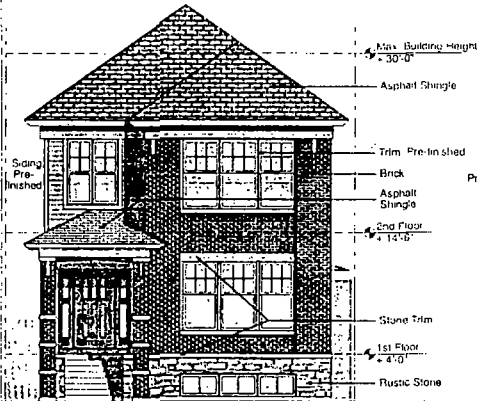
30 ft Lot - Option 3
