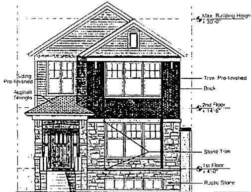
30 ft Lot - Option 1
