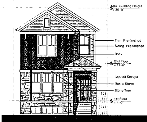
26 ft Lot - Option 1
