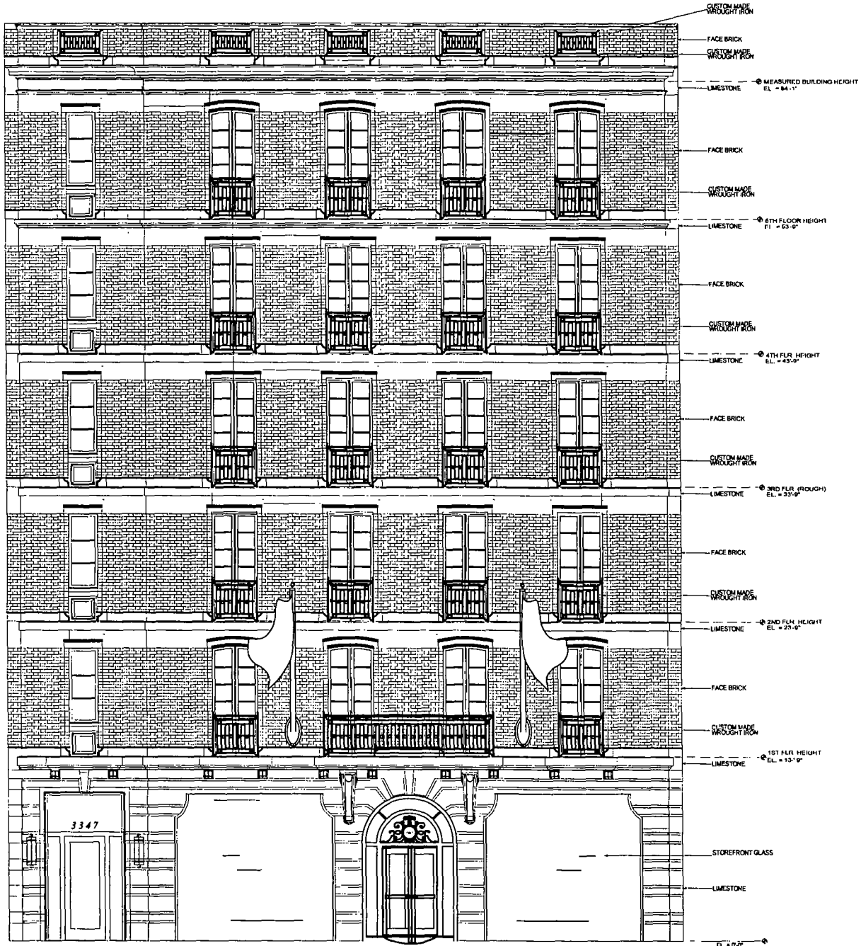
WEST ELEVATION
