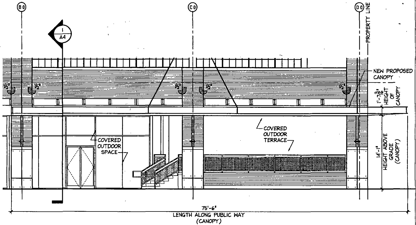
ELEVATION OF PROPOSED CANOPY OVER PUBLIC WAY (N. OGDEN ST.)
