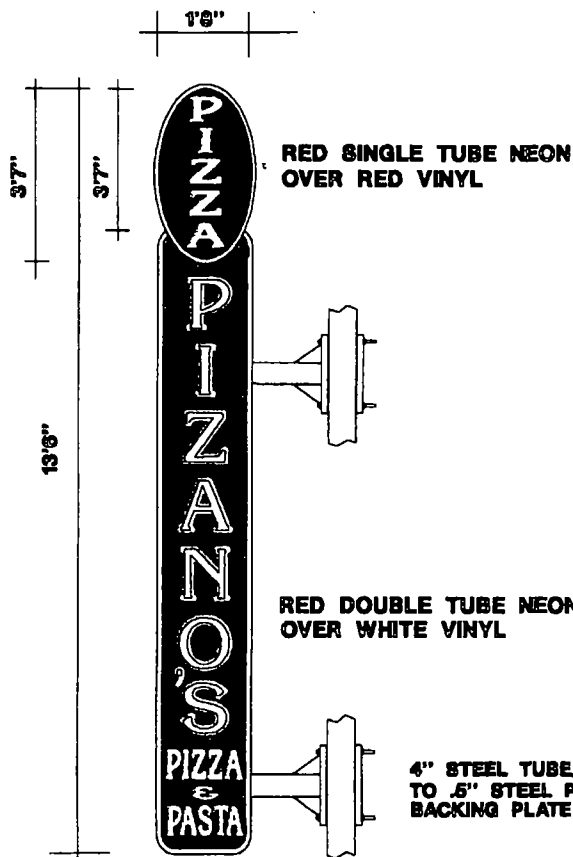
13'6"x1'8" PROJECTING SIGN
