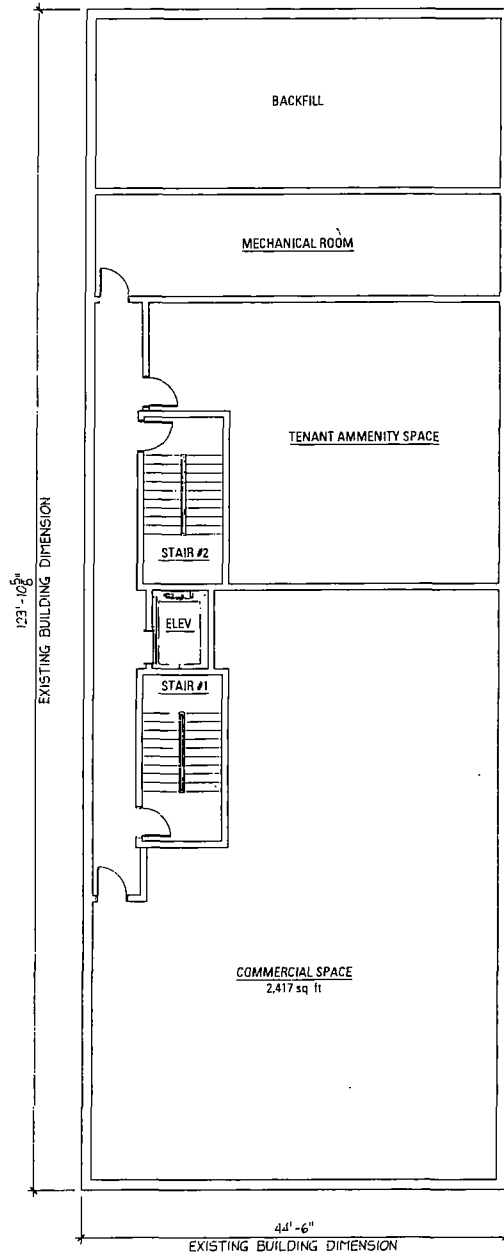
BASEMENT PLAN - (4,682 sq ft)
