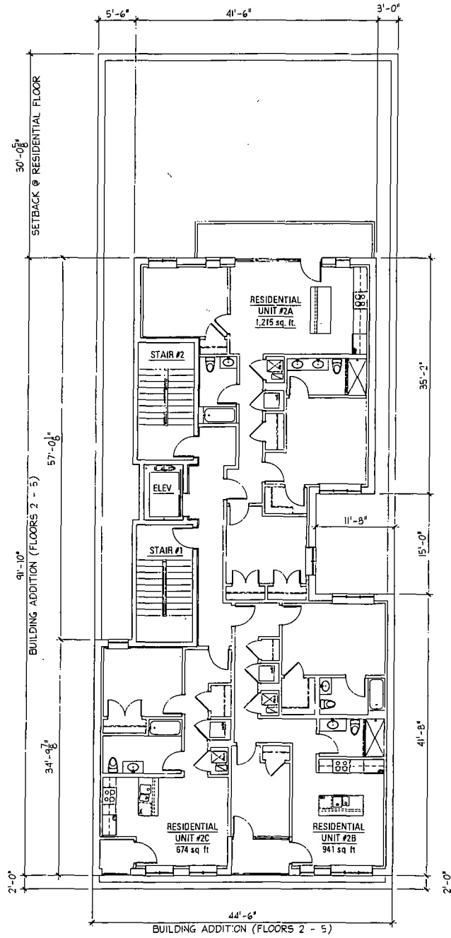
SECOND FLOOR PLAN 3,414 SQ. FT.
