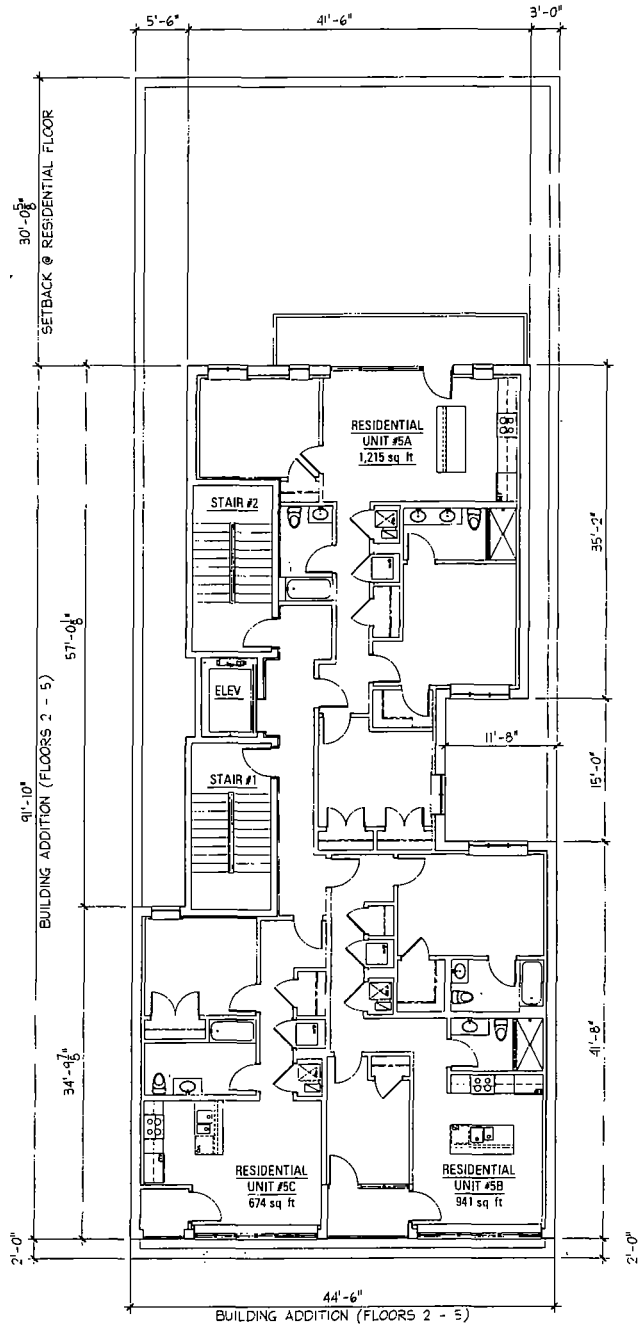
FIFTH FLOOR PLAN 3,414 SQ. FT.
