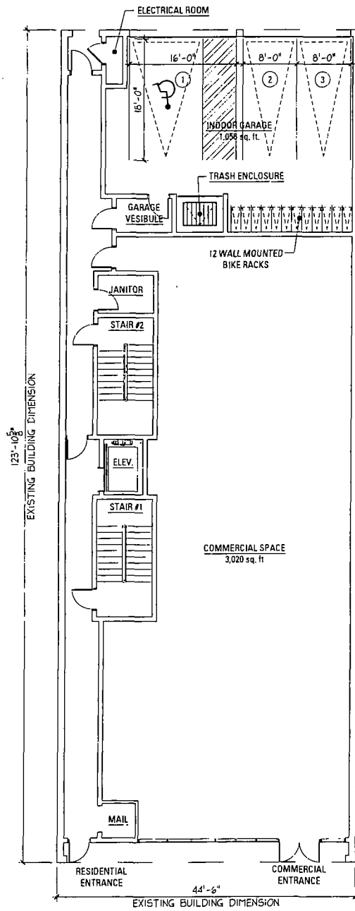
FIRST FLOOR PLAN 5,513 GROSS SQ. FT. (4,456 F.A.R. SQ. FT.) 3/32" = 1'-0"
