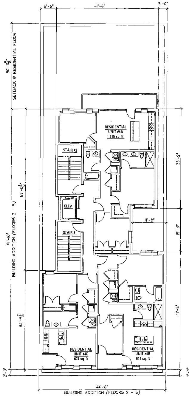
FOURTH FLOOR PLAN 3,414 SQ. FT.
