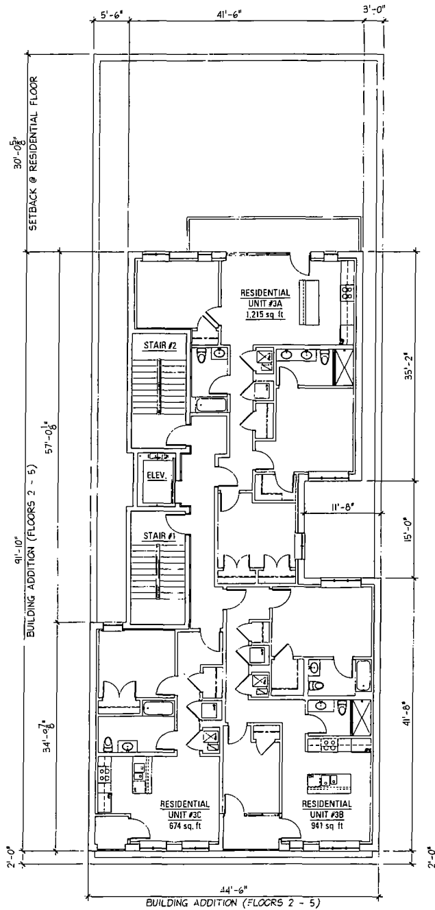
THIRD FLOOR PLAN 3,414 SQ. FT.
