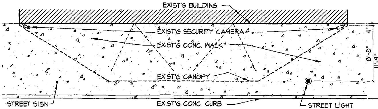
EXISTING PLAN 1/8"=1'-0"
