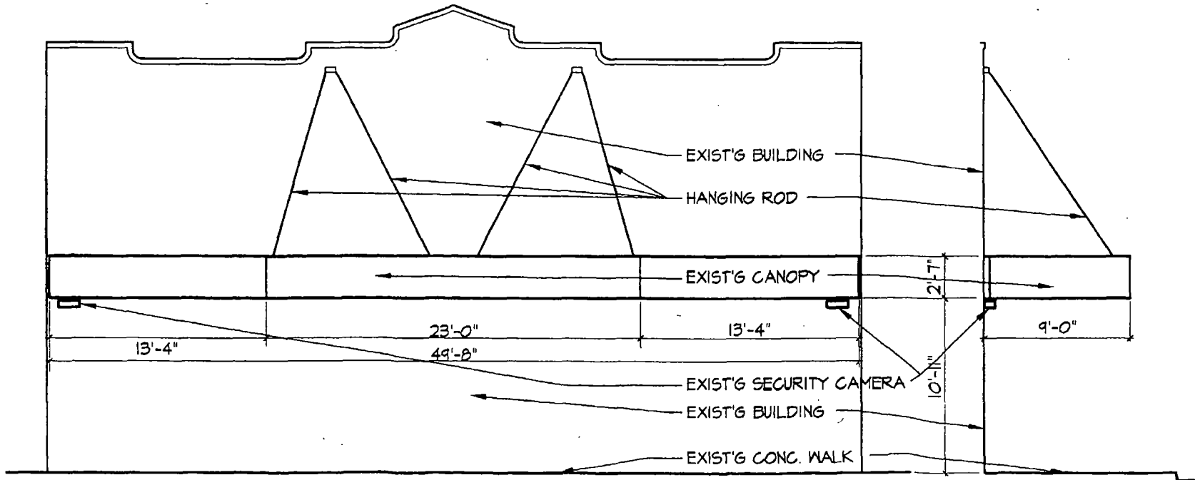
FRONT ELEVATION 1/8"=1'-0"
