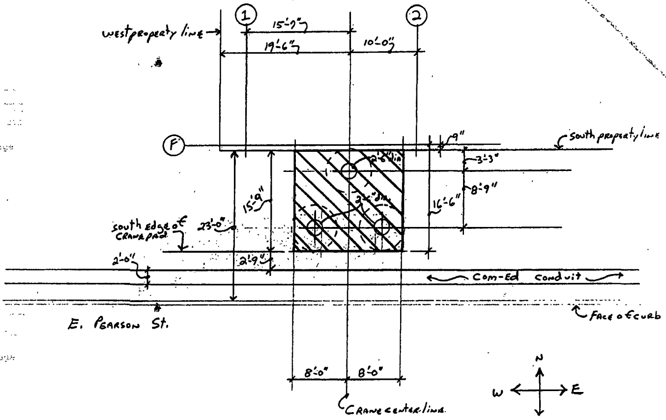
Temporary Construction Tower Crane Pad
