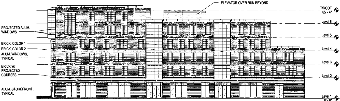
N-101 BUILDING - NORTHEAST ELEVATION Scale: N.T.S.
