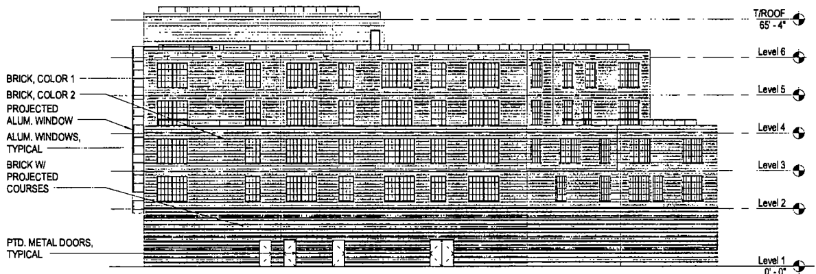
N-101 BUILDING - NORTHWEST ELEVATION Scale: N.T.S.
